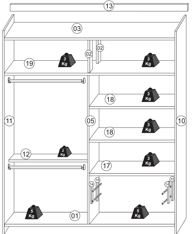
Vista frontal Vista frontal/Front view
